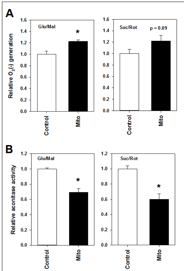
Figure 2. (A) Superoxide generation from mitochondria isolated from muscle of wild type (Control) and TgMito MsrA (mito) mice provided glutamate and malate (Glu/Mal) or succinate and rotenone (Suc/Rot). (B) Aconitase activity in isolated mitochondria provided glutamate and malate (Glu/Mal) or succinate and rotenone (Suc/Rot). Bars represent average values for n=6 for each group \pm SEM. Asterisks indicate significant difference as measured by t-test ( p < 0.05 ).
