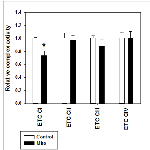
Figure 3. Electron transport chain complex activity in isolated mitochondria from wild type (Control) and TgMito MsrA mice (Mito). Bars represent average values for given complex for n=5 for each group \pm SEM. Asterisks indicate significant difference as measured by t-test ( p < 0.05 ).
