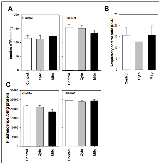
Figure 4. (A) ATP production from isolated mitochondria provided glutamate and malate (Glu/Mal) or succinate and rotenone (Suc/Rot). (B) Respiratory control ratio (RCR) of mitochondria provided glutamate and malate. (C) Membrane potential of isolated mitochondria provided glutamate and malate (Glu/Mal) or succinate and rotenone (Suc/Rot). Skeletal muscle mitochondria was isolated from wild type (Control), TgMito MsrA (Mito) and TgCyto MsrA (Cyto) mice. Bars represent average values for n=5 for each group \pm SEM. Asterisks indicate group differs significantly from others by ANOVA ( p < 0.05 ).
