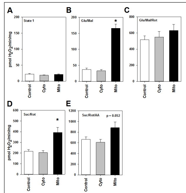
Figure 1. Mitochondrial production of H 2 O 2 with no substrates provided (A; state 1) or provided with glutamate and malate (B; Glu/Mal), glutamate, malate and rotenone (C; Glu/Mal/Rot), succinate and rotenone (D; Suc/Rot) or succinate, rotenone and antimycin A (E; Suc/Rot/AA). Skeletal muscle mitochondria was isolated from wild type (Control), TgMito MsrA (Mito) and TgCyto MsrA (Cyto) mice. Bars represent average values for n=5 for each group \pm SEM. Asterisks indicate group differs significantly from others by ANOVA ( p < 0.05 ).
